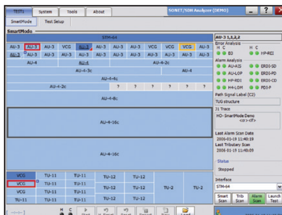
■ FTB-8120NGE/8130NGE SmartMode: multichannel signal discovery with real-time alarm scan (shown in the FTB-500 user interface).
