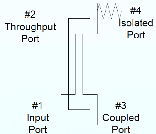
Figure 2. Example of a Typical Directional Coupler Schematic
