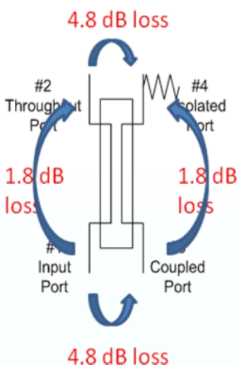
Figure 3. A 4.8/1.8 dB Coupler
